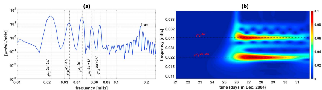
Figure 6. (a) Power spectral density of the synthetic GRACE range-rate perturbations due to the {}_0S_2 mode focused at lower frequencies, and (b) 2-D time-frequency map of the synthetic range-rate data from 21 to 31 December 2004 obtained using the wavelet analysis.
